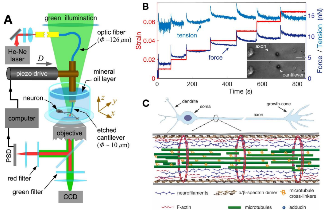
Fig: Probing axonal mechanics using home-built Micro-Extension Rheometer reveals strain-softening in axons that protect neurons from damage via reversibly unfolding of spectrin repeated units.
