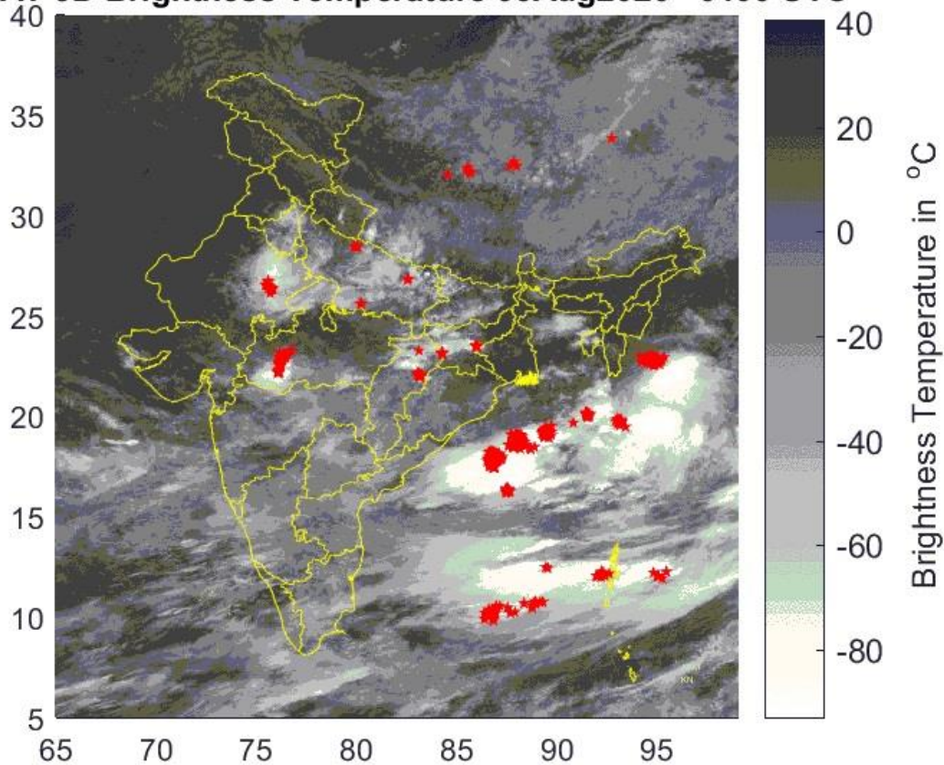
INSAT 3D Brightness Temperature 03Aug2020 0400 UTC
