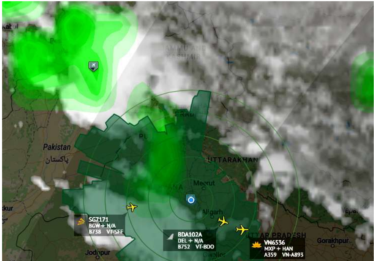
Frequent streams of western disturbances crossing northern India observed [as of 11 th May, 2020 8:31 PM]
